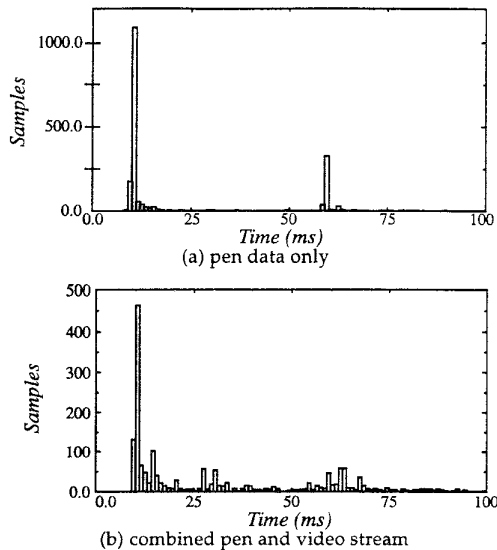
Figure 6: Round-trip latency measurements
