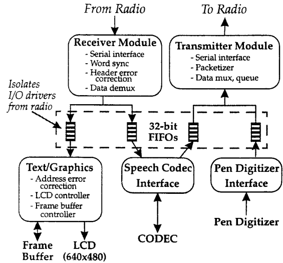
Figure 3: Block diagram of the protocol chip
