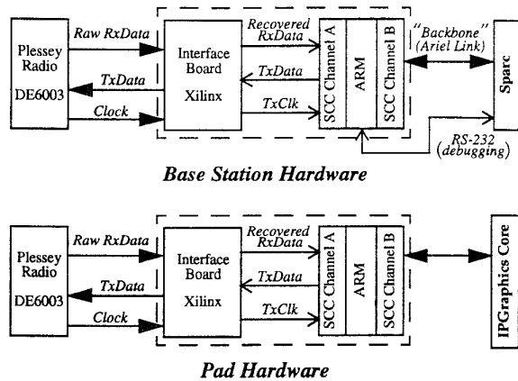
Figure 4: Hardware Block Diagram
