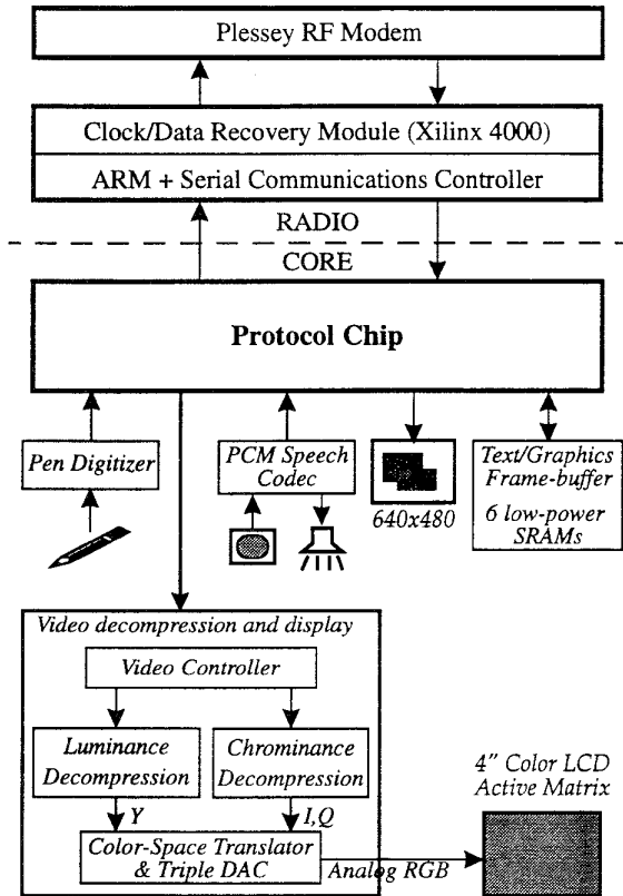
Figure 2: Overview of the InfoPad I/O Terminal
