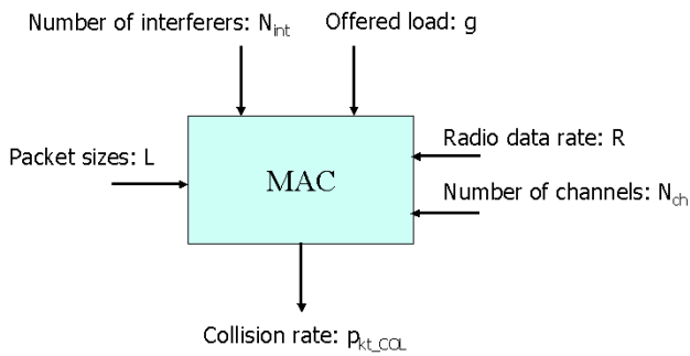
Fig.2 MAC model
