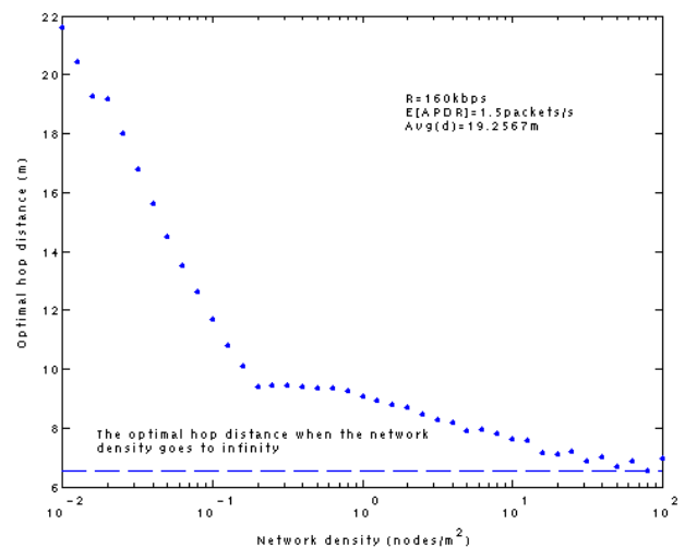
Fig.11 Optimal hop distance as a function of the network density
