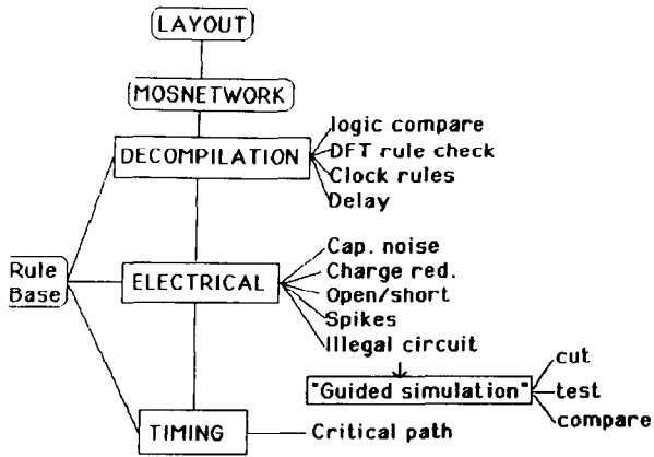
Fig. 4 : Overview of the DIALOG Verification system.
