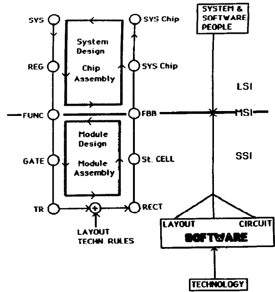
Fig. 1 : The meet-in-the-middle design methodology.
