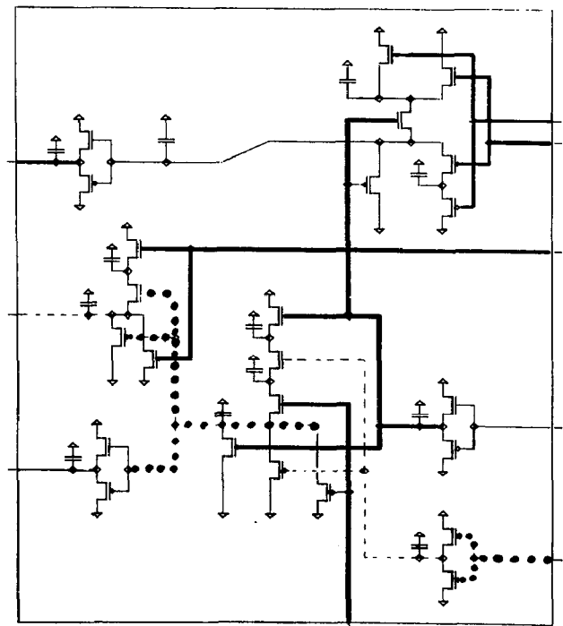
Fig. 7 : Automatic identification of critical path and required test pattern.
