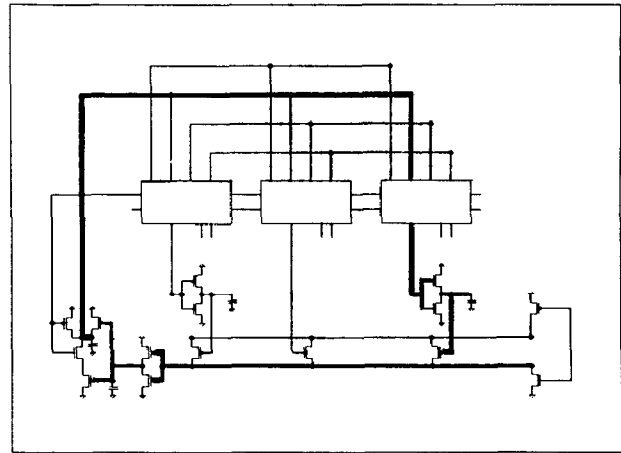
Fig. 5 : Example of a loop detected by DIALOG.
