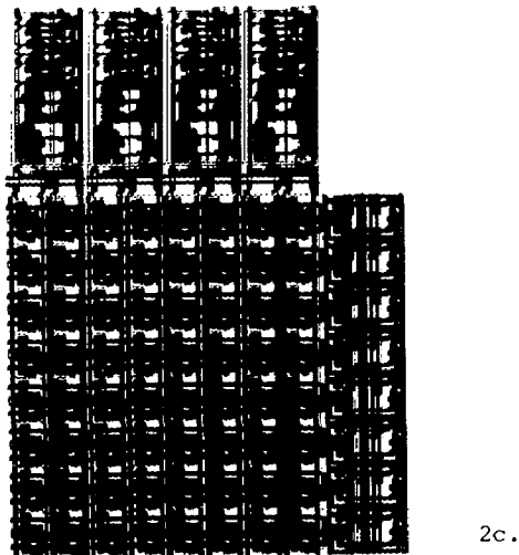
Fig. 2 : Interactive built up of a parameterized RAM. a : The array of RAM cells b : Relative positioning of decoder multiplexer and sense amplifiers. c : Final RAM layout after automatic abutment.
