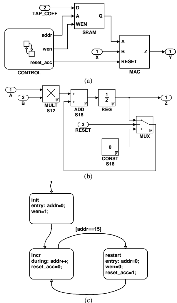
Figure 2: (a) Dataflow graphs of a time-multiplexed FIR Filter with (b) a detail of the multiply-accumulate block and (c) detail of the control logic finite state-machine.
