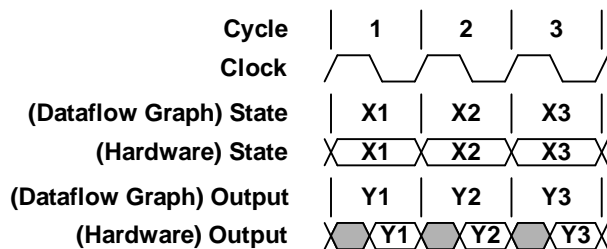
Figure 1: Dataflow-graph-to-hardware verification
