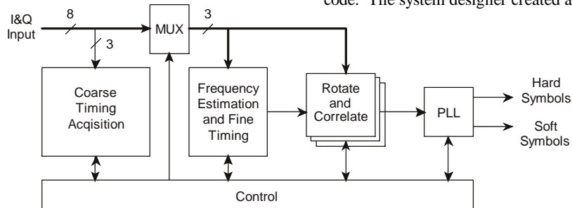
Figure 3: Block Diagram of the Baseband Receiver
