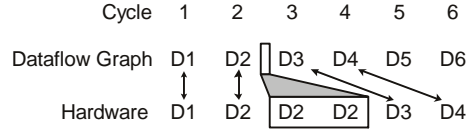
Figure 7: Don't-care windows to relax cycle-accuracy
