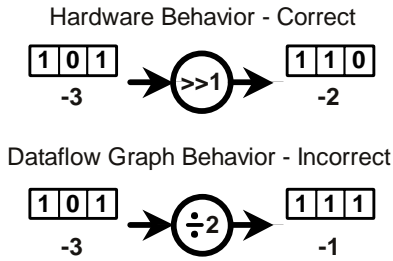
Figure 5: Constant-shift bit error problem
