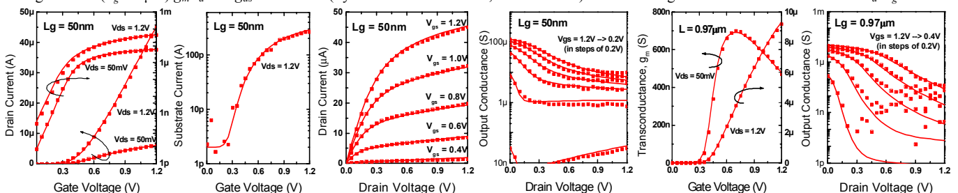
Fig. 9 Bulk FinFETs with moderate doping were fabricated with a TiN gate. Measured devices have T_{si} = 25\text{nm} and EOT = 1.95\text{nm} . Short channel ( L_g = 50\text{nm} ) fitting to measured I_d , I_{sub} and g_{ds} and long channel ( L_g = 0.97\mu\text{m} ) g_m and g_{ds} are shown. (Symbols: measured data, Lines: model) The model is able to describe both bulk FinFETs and SOI FinFETs.
