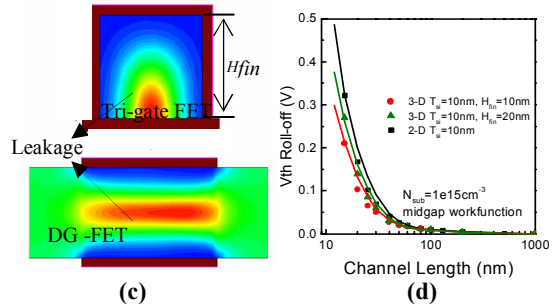
Fig. 7 Scalability of SCE model has been demonstrated through threshold voltage roll-off for different (a) oxide thickness and (b) body thickness for DG-FETs. (c) Leakage current path is different in tri-gate FETs due to 3D effects. (d) SCE model also exhibits fin height scalability for tri-gate FETs (Symbols: TCAD, Lines: Model)
