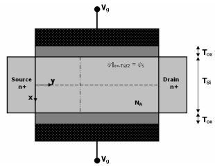
Fig. 2 Schematic of a symmetric DG-FET. In all comparisons with TCAD, T_{ox} = 2\text{nm} , T_{si} = 20\text{nm} , L_g = 1\mu\text{m} and metal gate with mid-gap work-function has been used unless specified.
