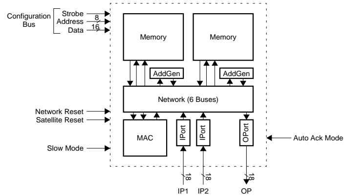
Fig. 1. Block Diagram of the P1 Prototype
