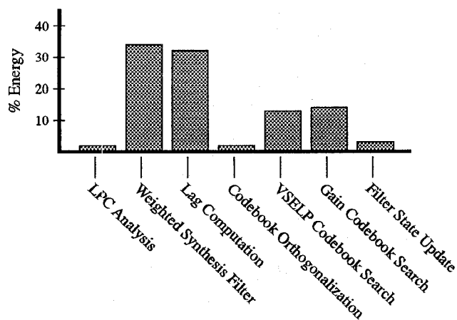
Figure 2: Arithmetic Energy Profile for the VSELP Speech Coder
