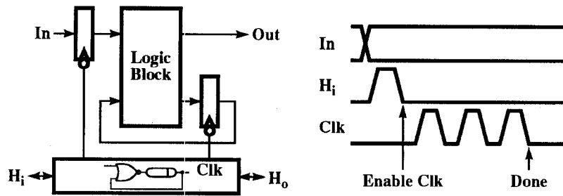
Figure 7: Locally Synchronous, Globally Asynchronous Timing Scheme
