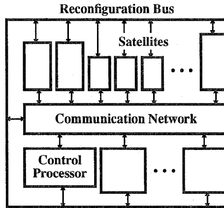
Figure 3: Architecture Template
