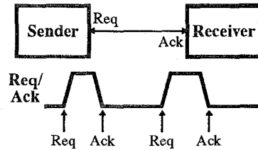
Figure 6: Single-Wire, Two-Phase Asynchronous Handshaking Protocol
