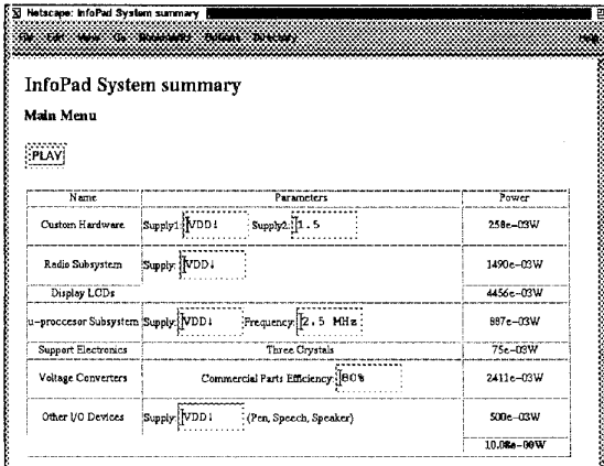
Figure 5 InfoPad system power breakdown
