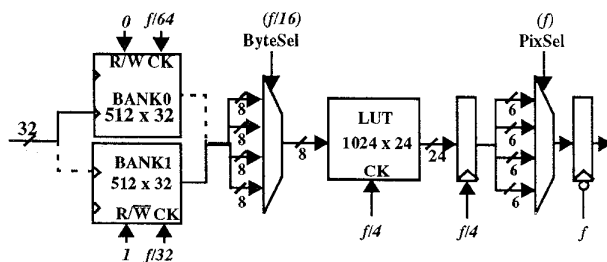
Figure 3 Alternate implementation of the decompression chip
