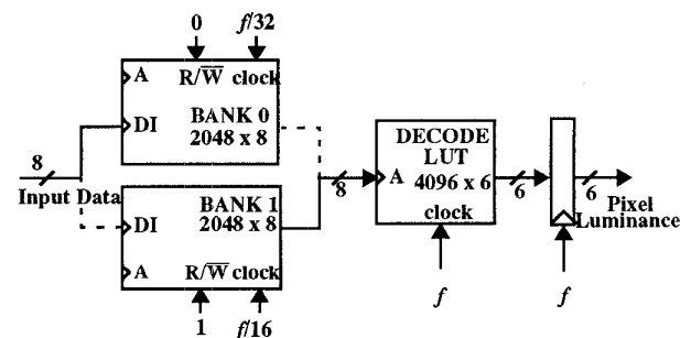
Figure 1 Block diagram of a luminance decompression chip
