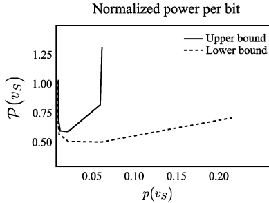
Fig. 4. Bounds on \mathcal{P}(v_S) : The minimum values of upper and lower bounds are 40% and 49% lower than the worst-case.
