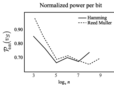
Fig. 5. \mathcal{P}(v_S) for finite n : For an outage \epsilon = 0.01 , the optimum power reduction for Hamming and Reed Muller codes are plotted.
