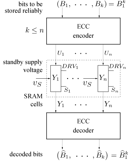
Fig. 3. Standby-SRAM architecture: Let B_1^k be the data vector to be stored. Then B_1^k is encoded into U_1^n and stored in n memory cells. The i^{\text{th}} stored bit is stuck-at S_i if DRV_i \geq v_S , otherwise U_i is read-out. The decoder reads Y_1^n and outputs \hat{B}_1^k . The voltage v_S is selected such that \mathbb{P}(\text{outage}) negligible (see (2)).
