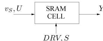
Fig. 2. Standby SRAM cell: The SRAM cell has two statistically independent parameters: (i) a time-invariant positive continuous-valued threshold-voltage DRV , and (ii) a binary bias-state S \in \{0, 1\} . The inputs are the supply voltage v_S and a bit U \in \{0, 1\} to be stored. The output is Y = U if v_S > DRV and S otherwise.
