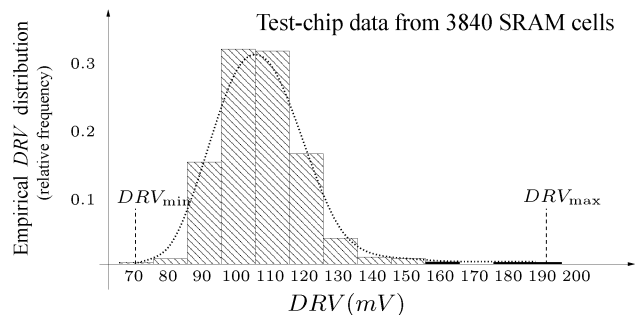
Fig. 1. Empirical DRV -distribution: The intra-chip DRV varies from 70 to 190mV for the 90nm CMOS technology. The dotted curve is a smooth fit to the empirical DRV -distribution [1].
