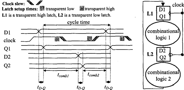
Figure 10: Skew-tolerant level sensitive clocking [15].
